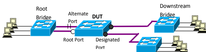
Figure 1. An example of a Bridged Local Area Network supporting STP
