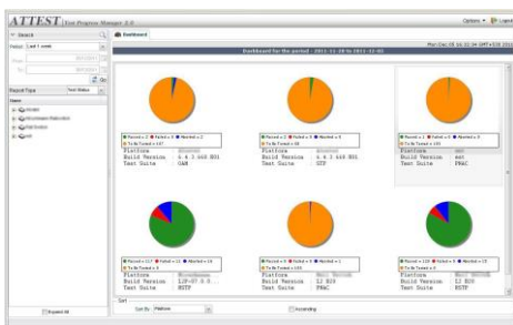
Figure 4: Testing Dashboard
