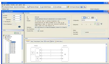
Figure 2: Testcase Manager
