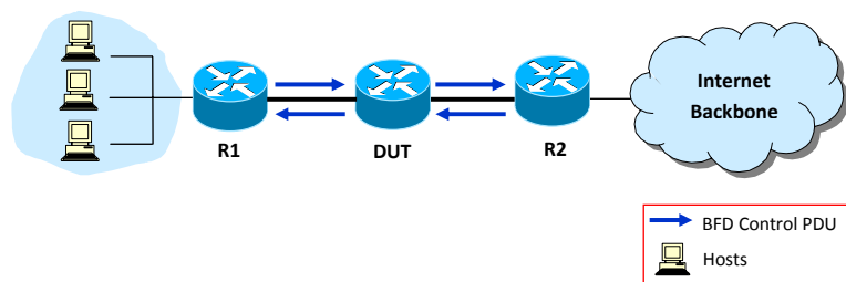
Figure 1. An Example of a network supporting BFD
